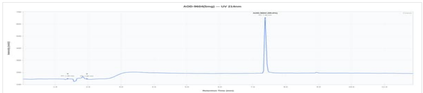
AOD-9604 5mg - 1: UV Chromatogram
