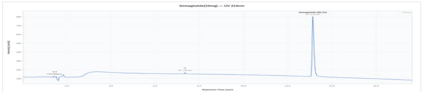
Semaglutide 10mg - 1: UV Chromatogram
